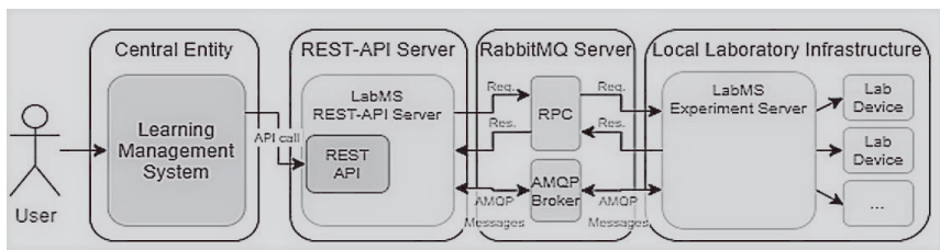
Figure 2. Combining AMQP and RPC protocols can enable communication for remote users with local laboratories without IP addresses (Adineh et al., 2022)
