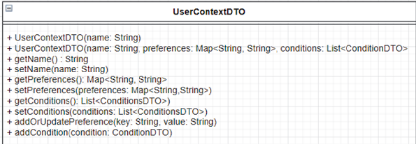
Figure 4: UML Diagram UserContextDTO
