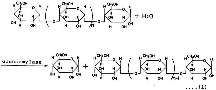
Figure 1. Glucoamylase-catalysed hydrolysis of terminal (1->4)-linked \alpha -D-glucose residues successively from non-reducing ends of the chains with release of \beta -D- glucose. 9
