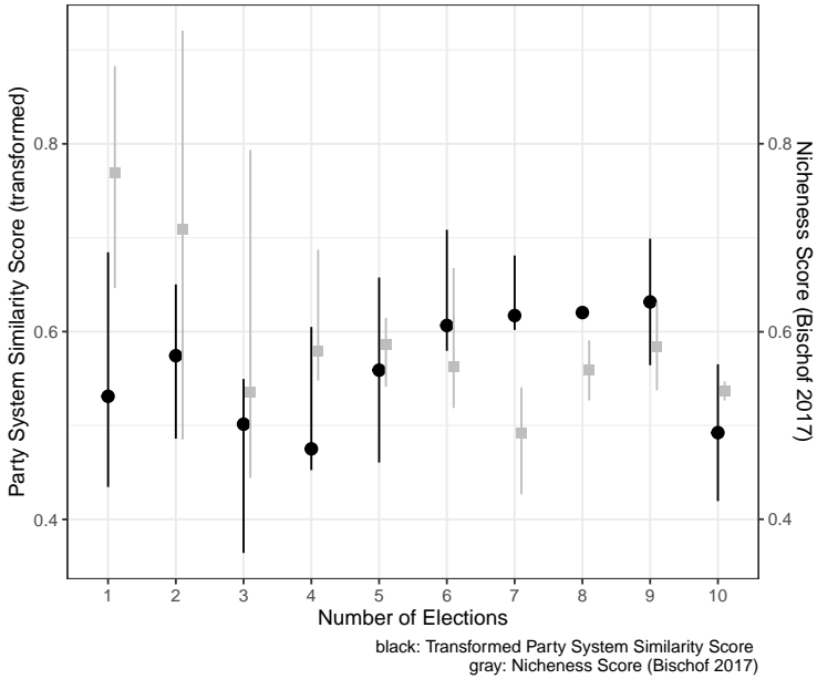
Figure 8.27: Nicheless Scores of Special Issue New Parties
