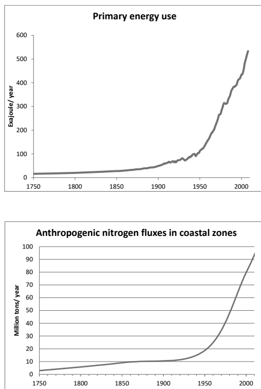
Charts: Primary energy use (socio-economic indicator) and anthropogenic input of nitrogen into coastal waters (ecological indicator) from 1750 to 2010 (Source: Will Steffen et al. 2015).
