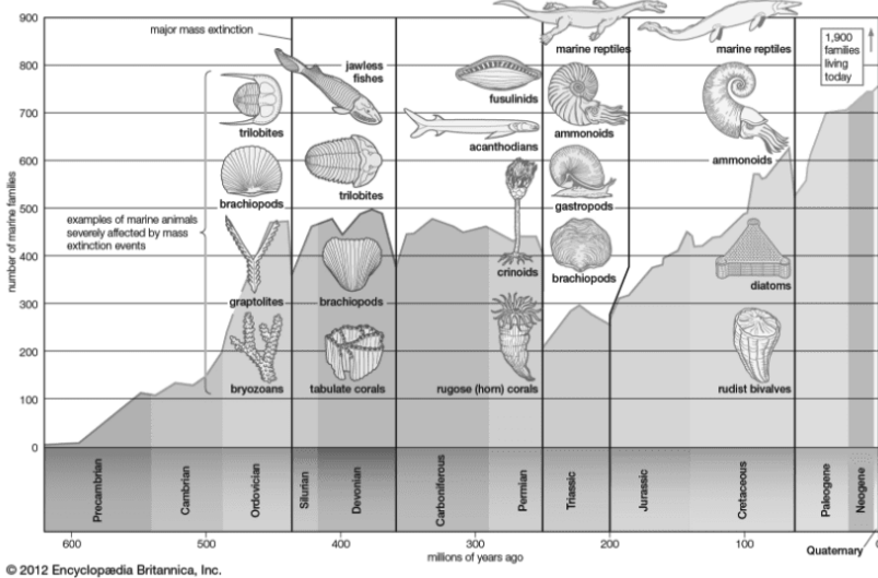
Diversity of marine animal families over geologic time
