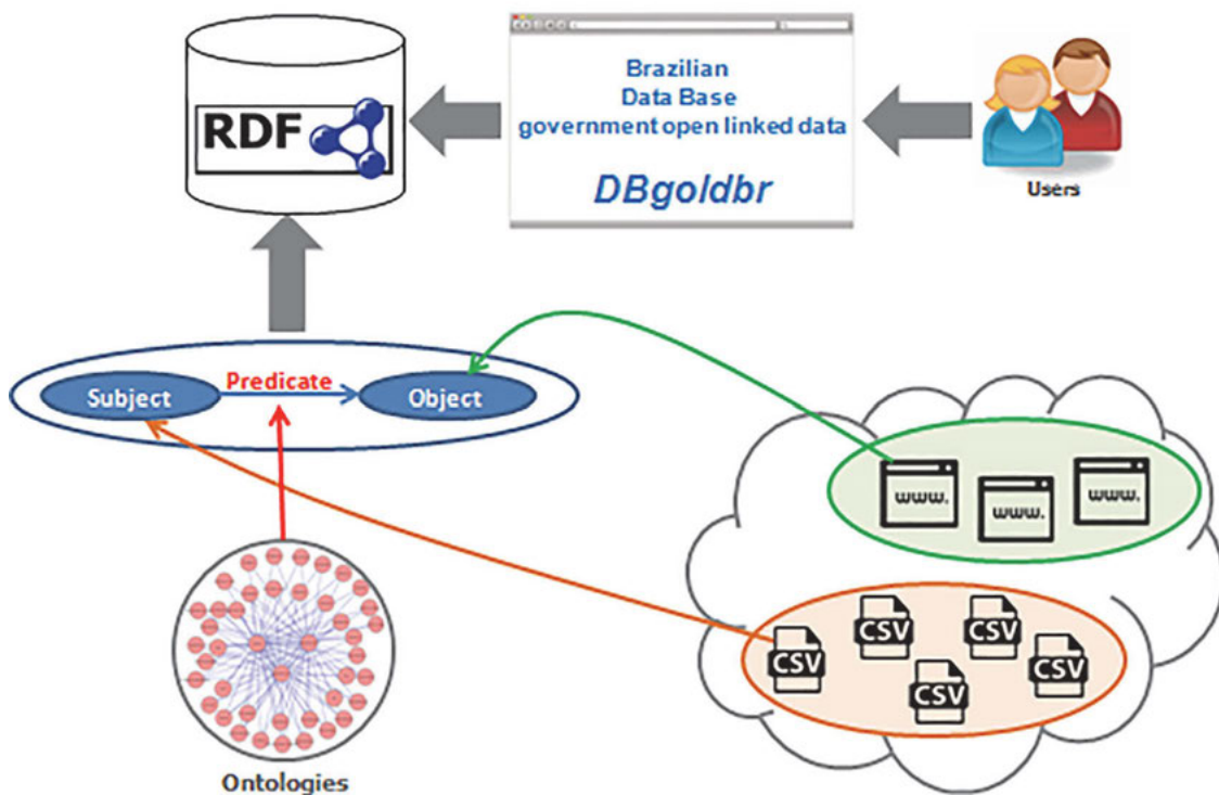
Figure 7. Using DBgoldbr to search for open data sources.
