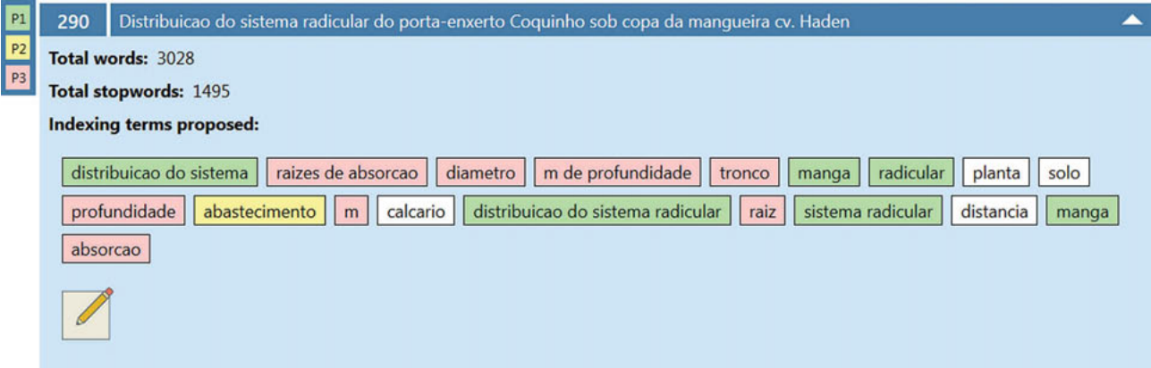
Figure 9. Indexing editing.
