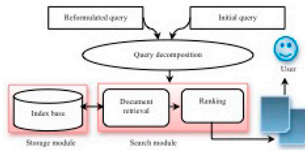
Figure 4. Search process architecture
